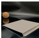
JS-B B-19 Metal section 规格SIZE6000*168.5*13.9
